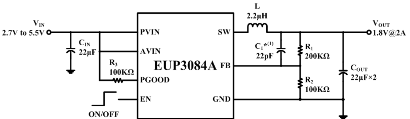
Figure 1. Application Circuit
