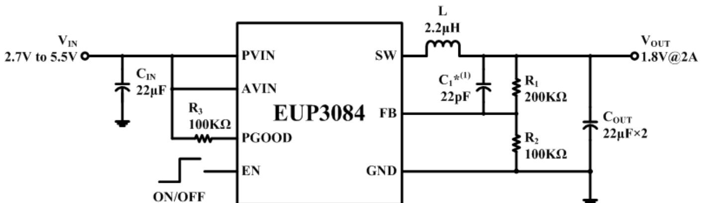
Figure 1. Application Circuit
